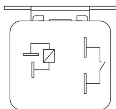
常开A型/Normally open A type
